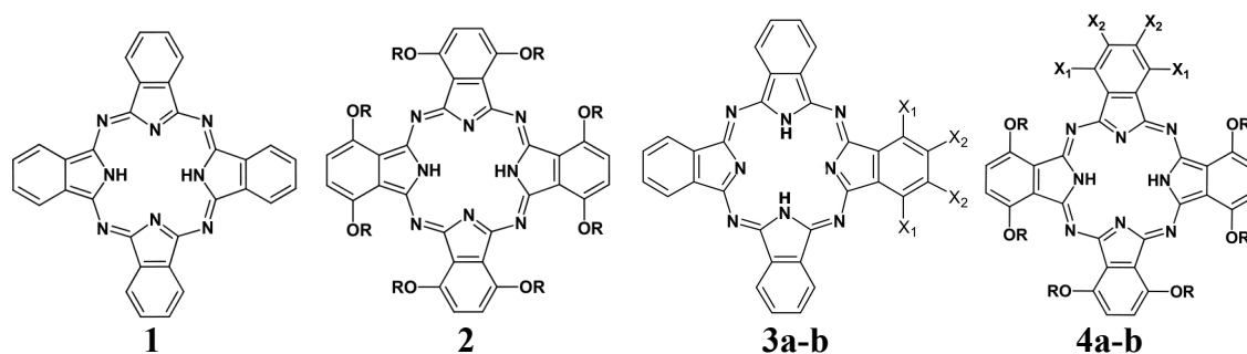
Fig. 1. The structural formulas of the compounds under study 1-4. a: X 1 = H, X 2 = Cl; b: X 1 = X 2 = Cl, R = C n H 2n+1 , n = 1-16
