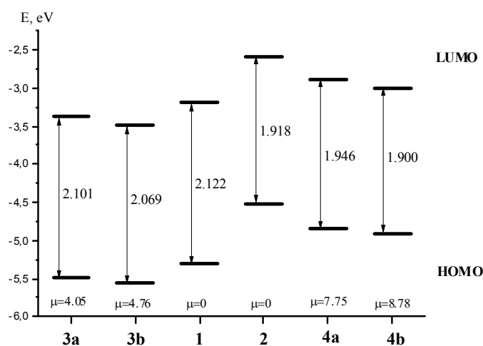
Fig. 3. The frontier orbitals energies for 1-4
