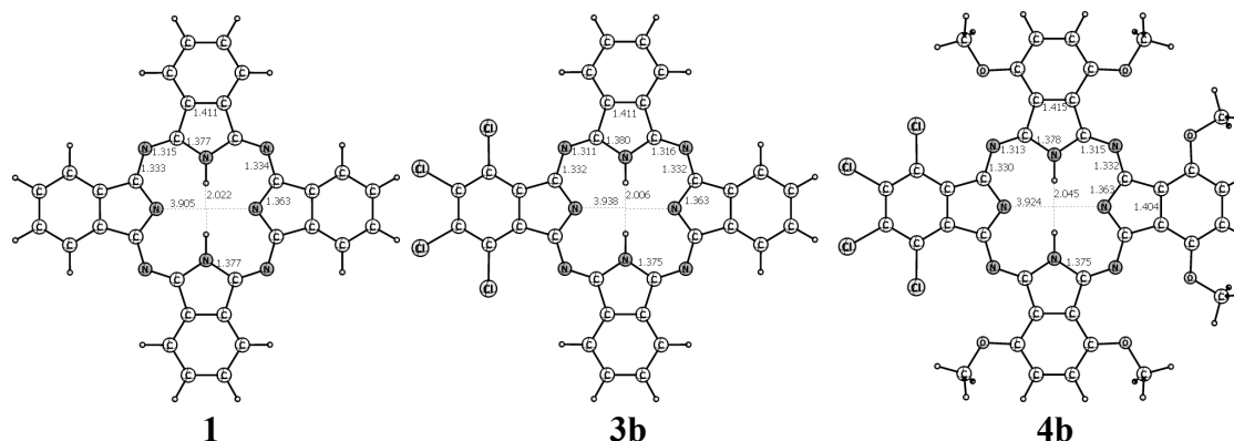
Fig. 2. Fragments of the internal cavity of the molecule of Compounds 1, 3b and 4b (n=1)
