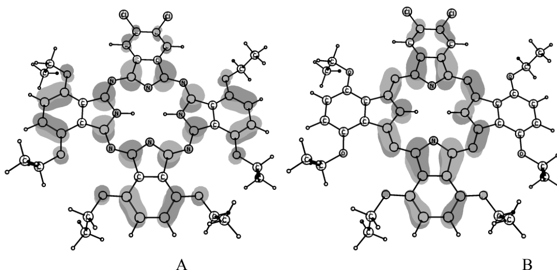
Fig. 4. View of HOMO (A) and LUMO (B) for 4a (n=2)
