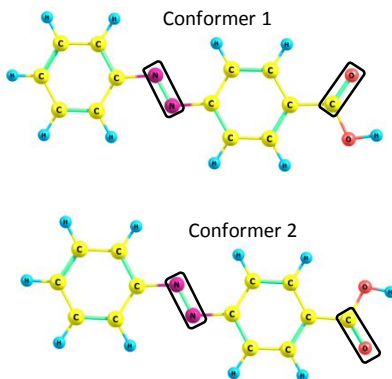
Fig. Geometric structure of 4-PABA conformers
