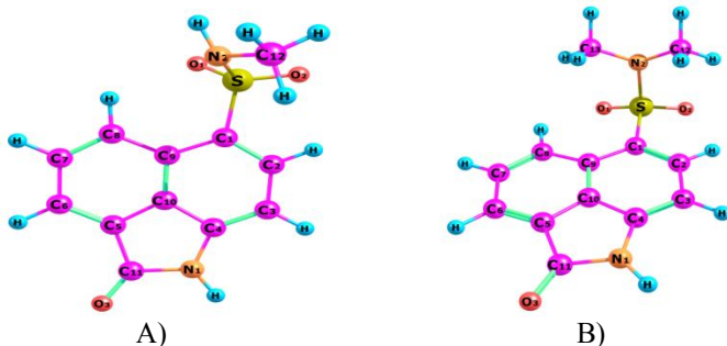
Fig. Geometric structure of the most stable conformers of the studied molecules
